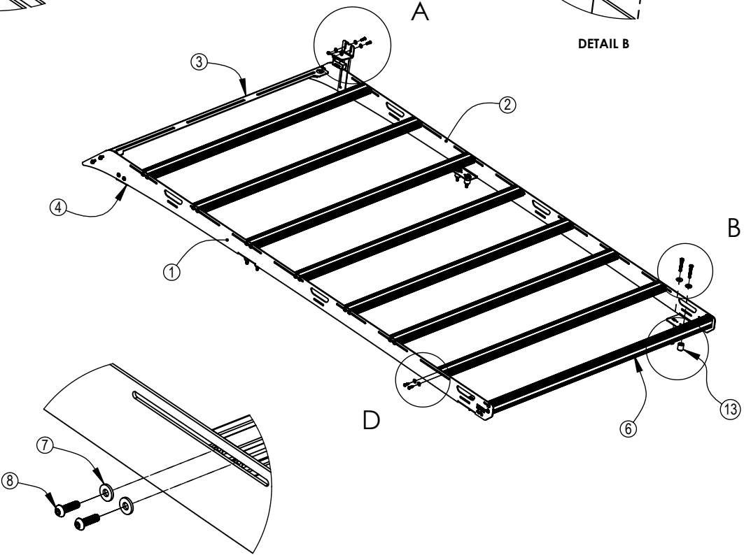
DETAIL D
